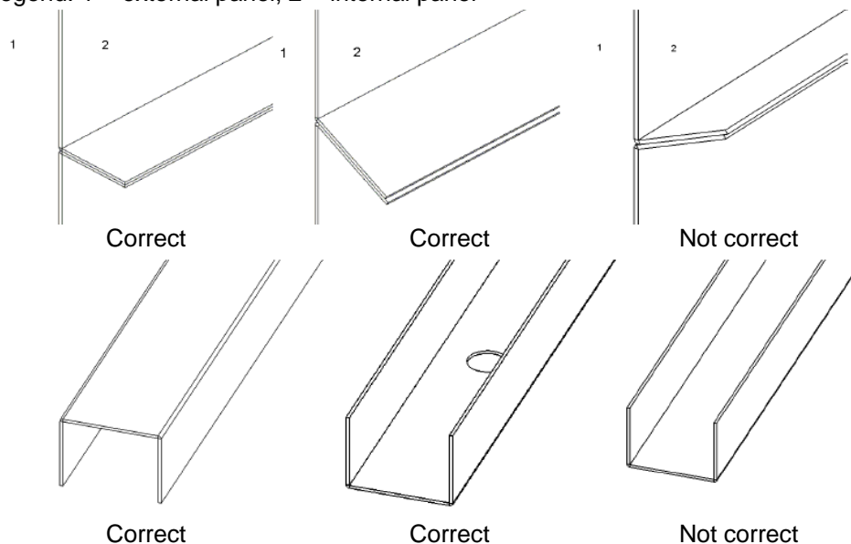
Internal assembly of the tower's vertical panels
