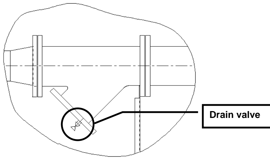
Example of a connection at right angle of the tube end
